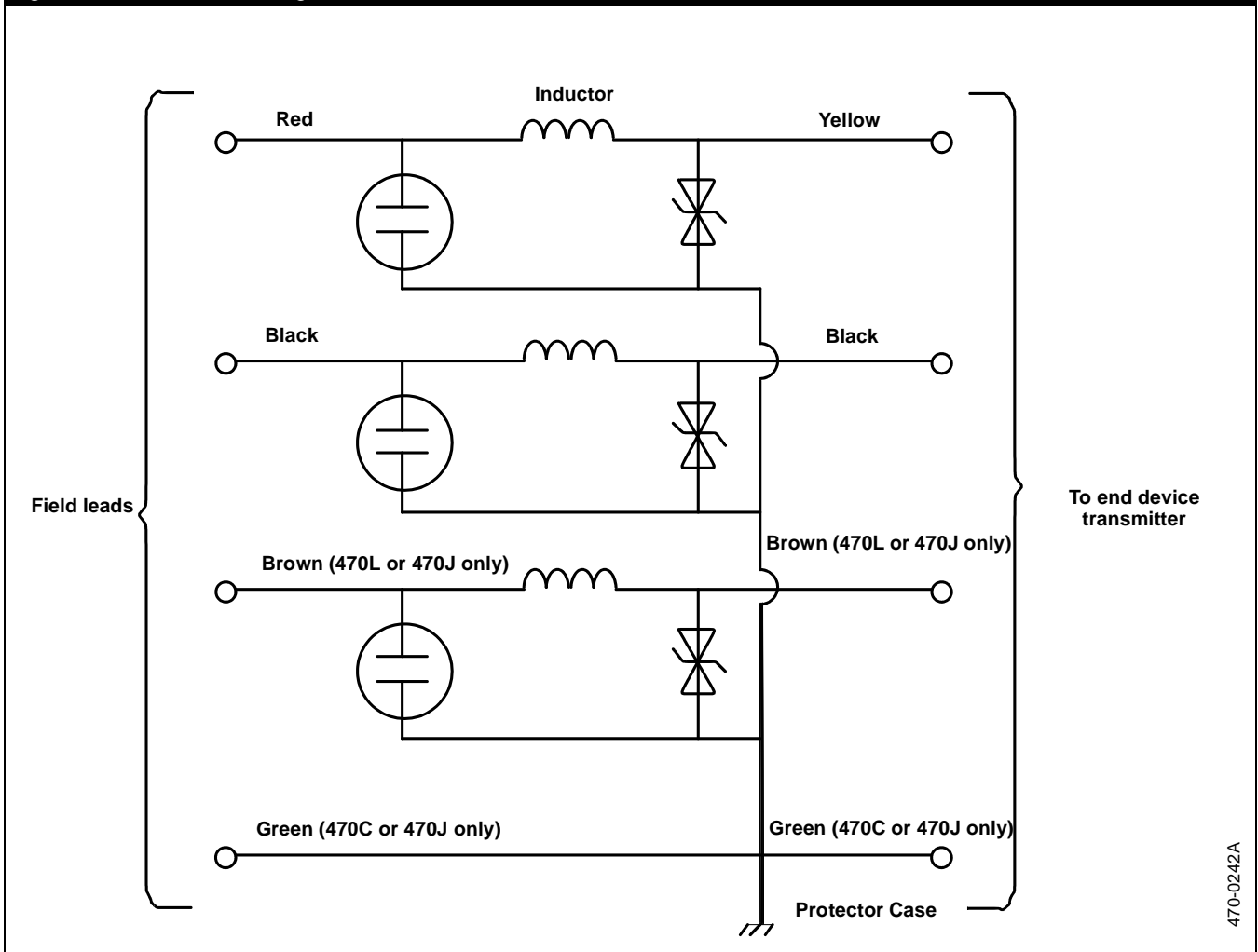
Figure 3-1. Schematic Diagram
